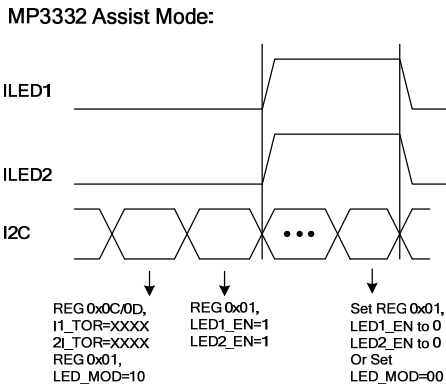
Figure 3: Assist Mode
