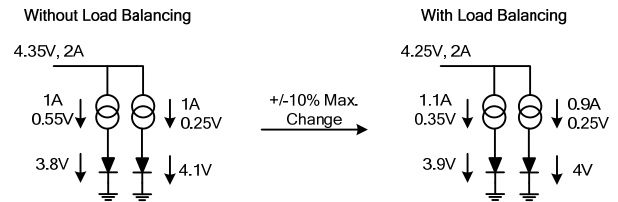
Figure 13: Load Balancing
