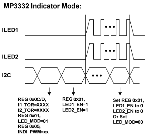
Figure 4: Indicator Mode
