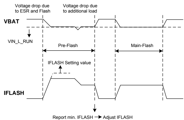
Figure 15: Pre-Flash Operation
