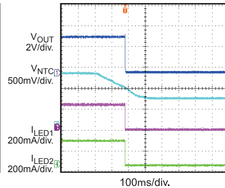
NTC Detection Set NTC_WD=0.88V
