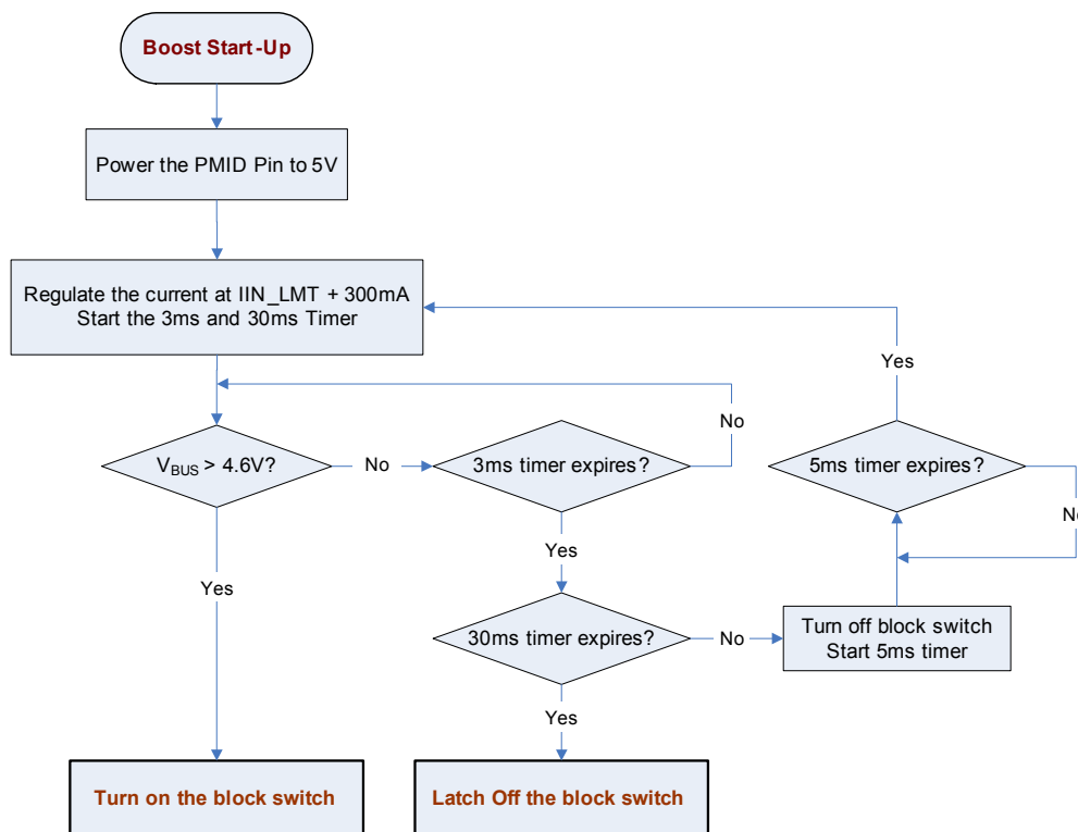
Figure 14: OTG Boost Start-Up Flow
