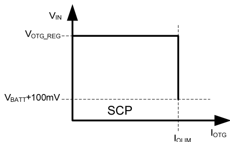
Figure 15. OTG Output U-I Curve
