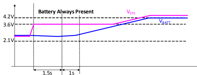
(b) Charging Start-Up with Battery Present
